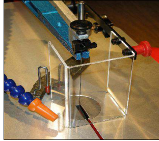
A7040 Blade guard
